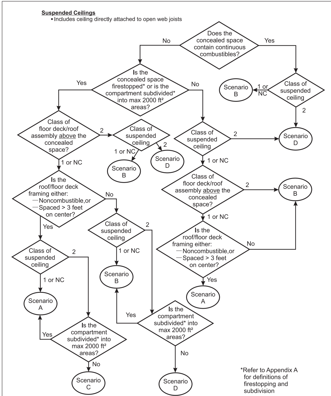
Fig. 2.2.2-1 Suspended ceilings
