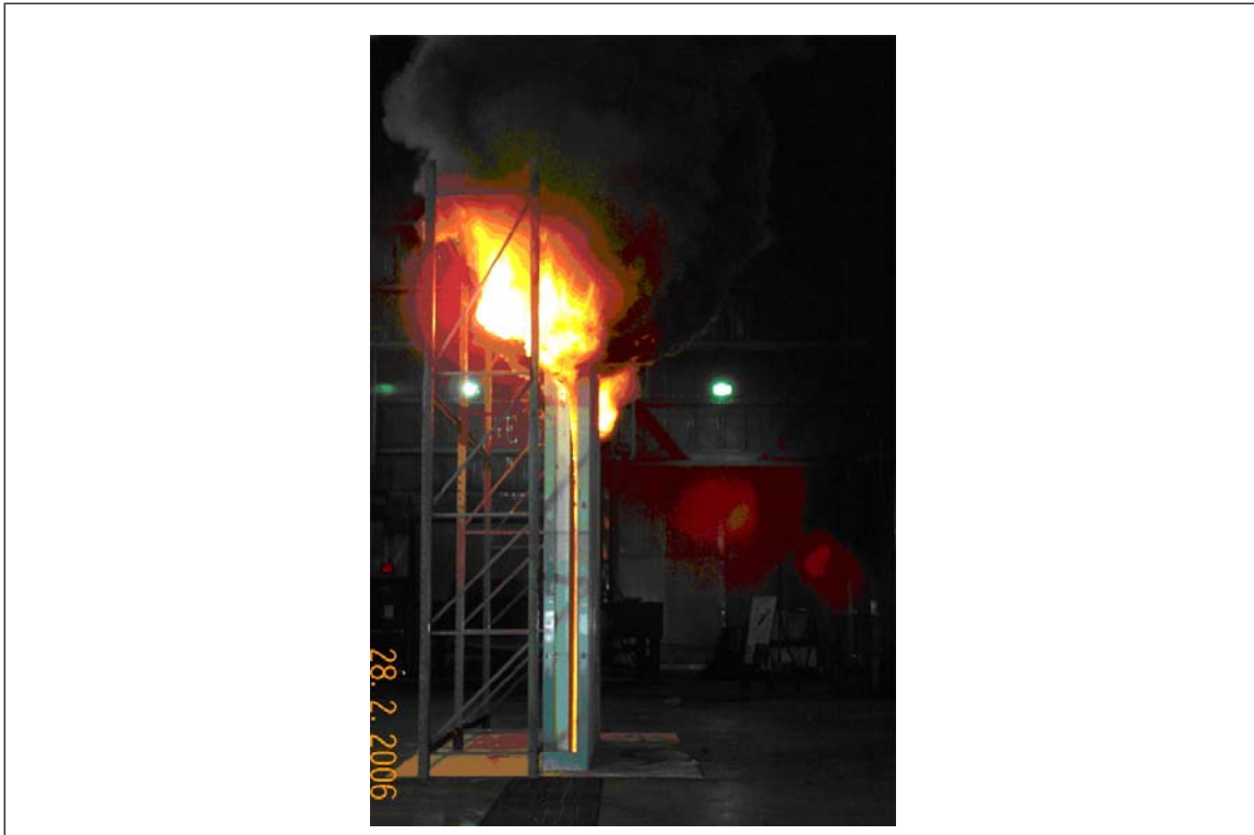
Fig. 3.3-1. Fire Test of cavity wall assembly using foam polystyrene insulation
