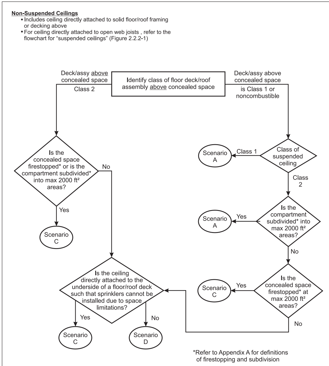
Fig. 2.2.2-2 Non-suspended ceilings
