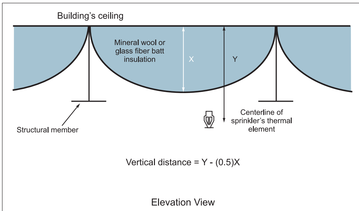
Fig. 25. Vertical distance between ceiling and centerline of sprinkler's thermal element in the presence of mineral wool or glass fiber batt insulation.
