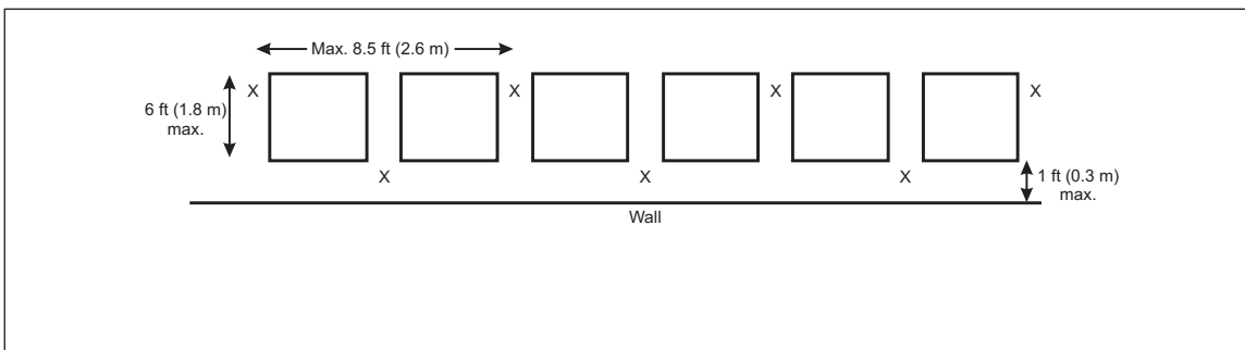
Fig. 19c. Plan view of alternative in-rack sprinkler arrangement for single-row racks up to 6 ft (1.8 m) deep located against wall
