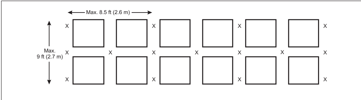
Fig. 20a. Plan view of alternative in-rack sprinkler arrangement for double-row racks up to 9 ft (2.7 m) deep
