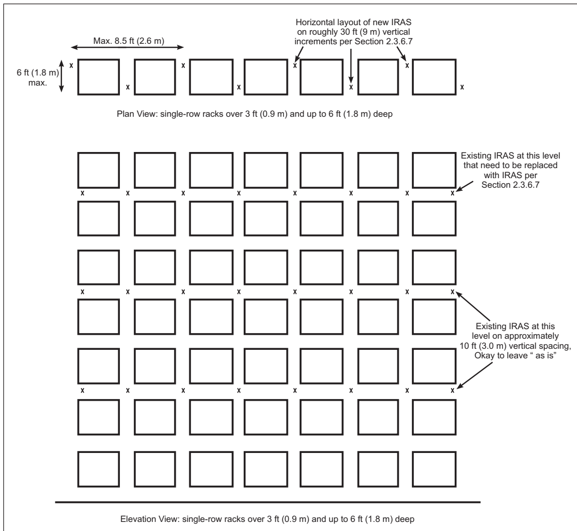
Fig. 23. Protection of uncartoned plastics in open-frame, single-row racks over 3 ft (0.9 m) and up to 6 ft (1.8 m) deep
