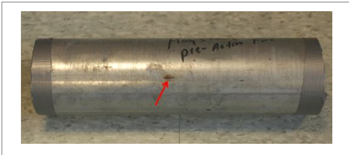
Fig. 13. Grooving corrosion of a longitudinal through-wall leakage in a galvanized steel pipe along its weld seam in a preaction
