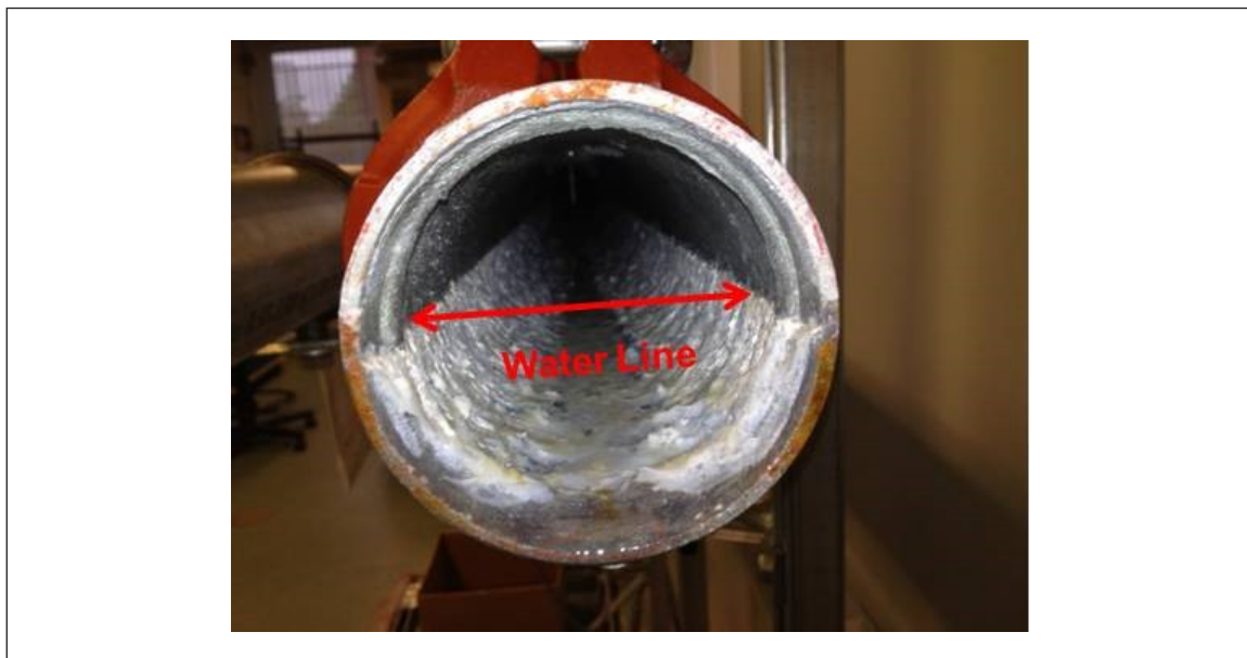
Fig. 4a. Galvanized steel pipe half-filled with tap water in house air after nearly six weeks' exposure
