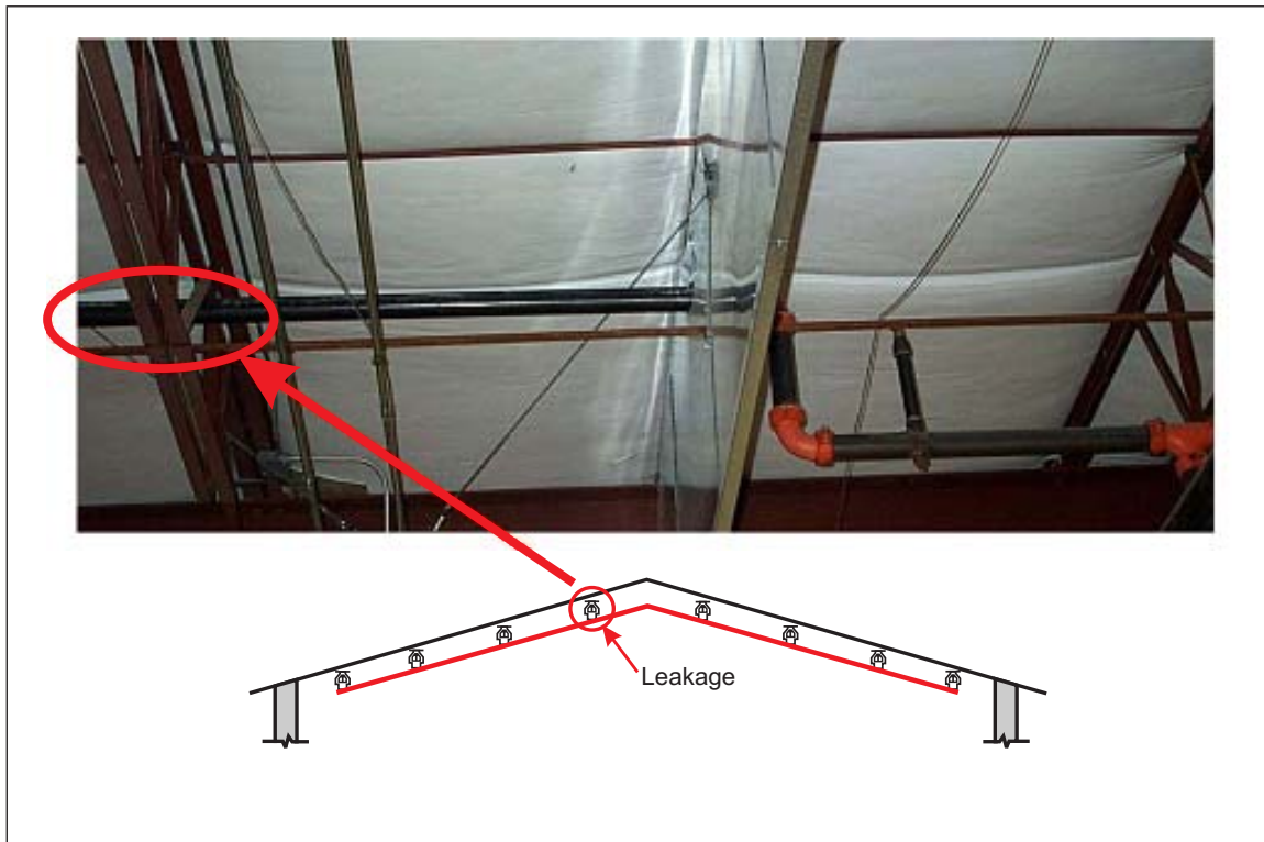
Fig. 6. Leakage sites of a wet pipe system due to trapped air
