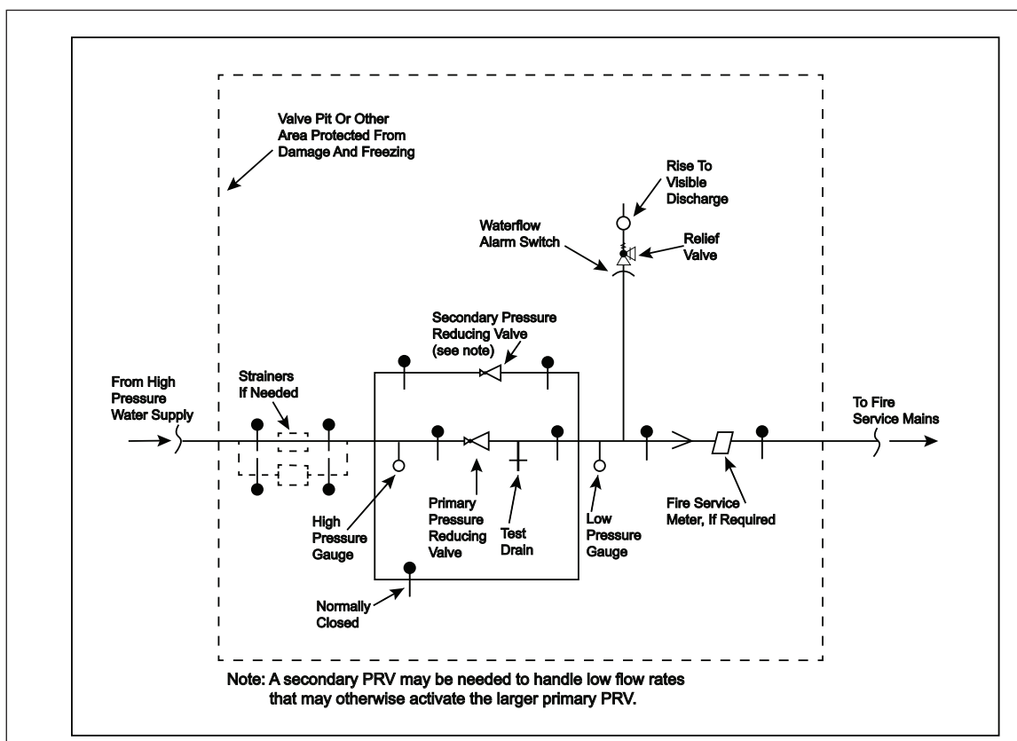
Fig. 2.3.1.6-1. Arrangement of pressure reducing valve for fire service
