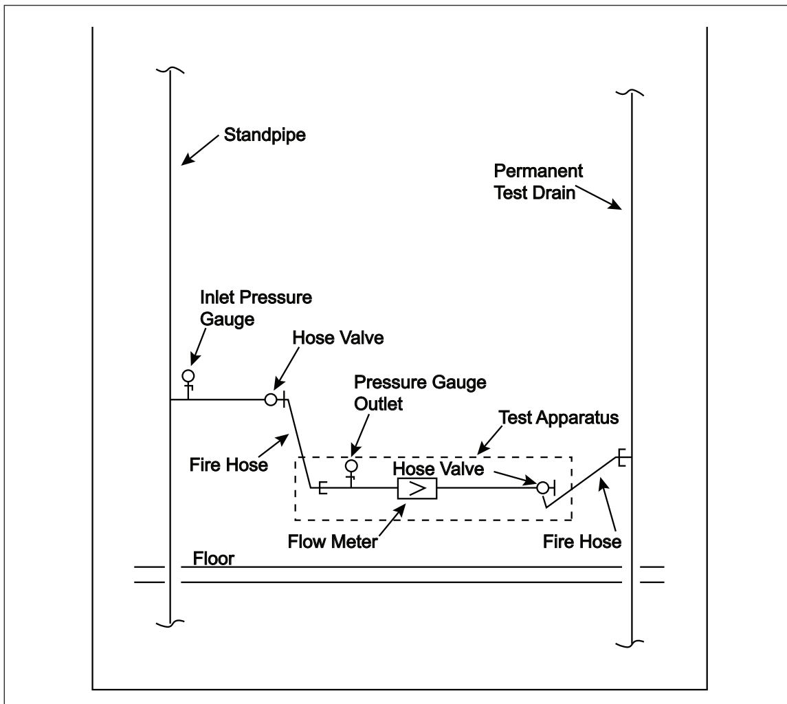
Fig. 2.3.3.1-1. Arrangement of annual full flow test on valves used in hose connections
