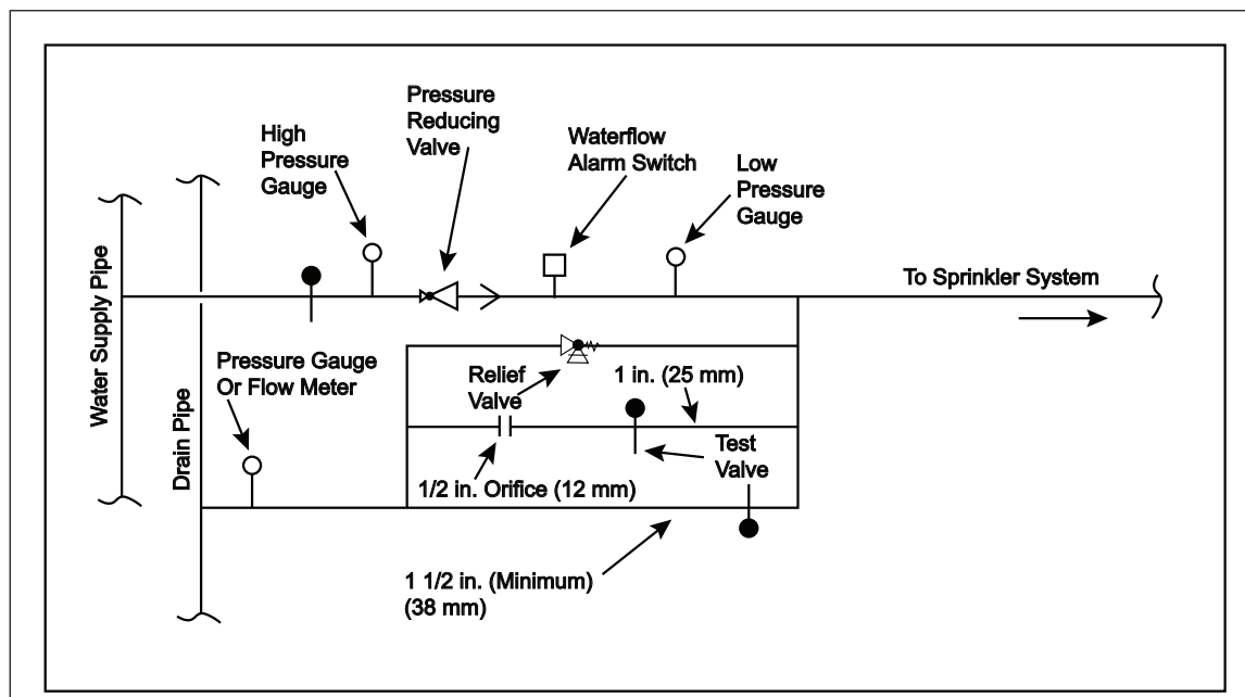
Fig. 2.3.2.1-1. Pressure reducing valve installation for individual sprinkler system (Note: A check valve is not needed for pressure reducing valves that have a check valve function incorporated in their design.)
