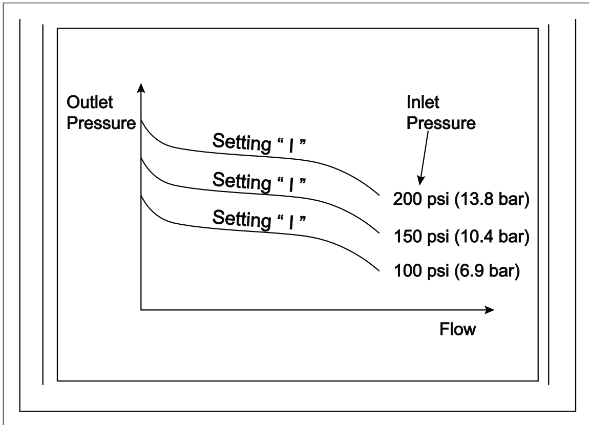
Fig. 3.3.1-2. Flow chart showing plot of outlet pressure versus flow rate through the valves for a given inlet pressure range
